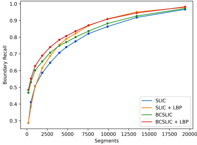
Fig. 14. Boundary performance with different methods on Dataset 1.
